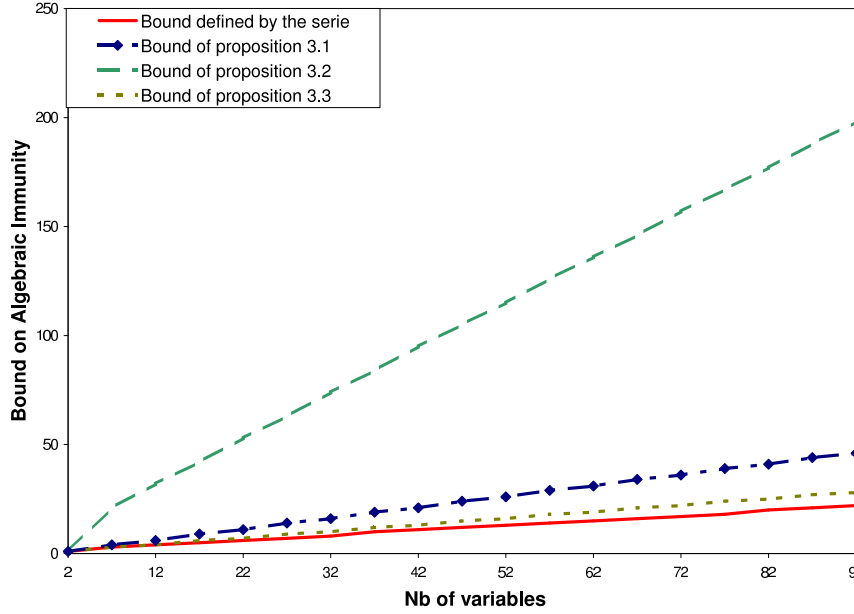
Figure 3: Comparison of bounds according to the number of variables
