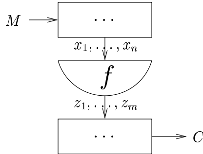
Block Cipher
