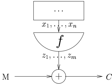
Stream Cipher
